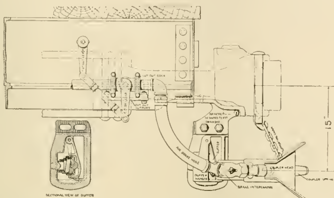
THE WESTINGHOUSE AUTOMATIC AIR AND STEAM COUPLER. SIDE ELEVATION. FREIGHT EQUIPMENT.
